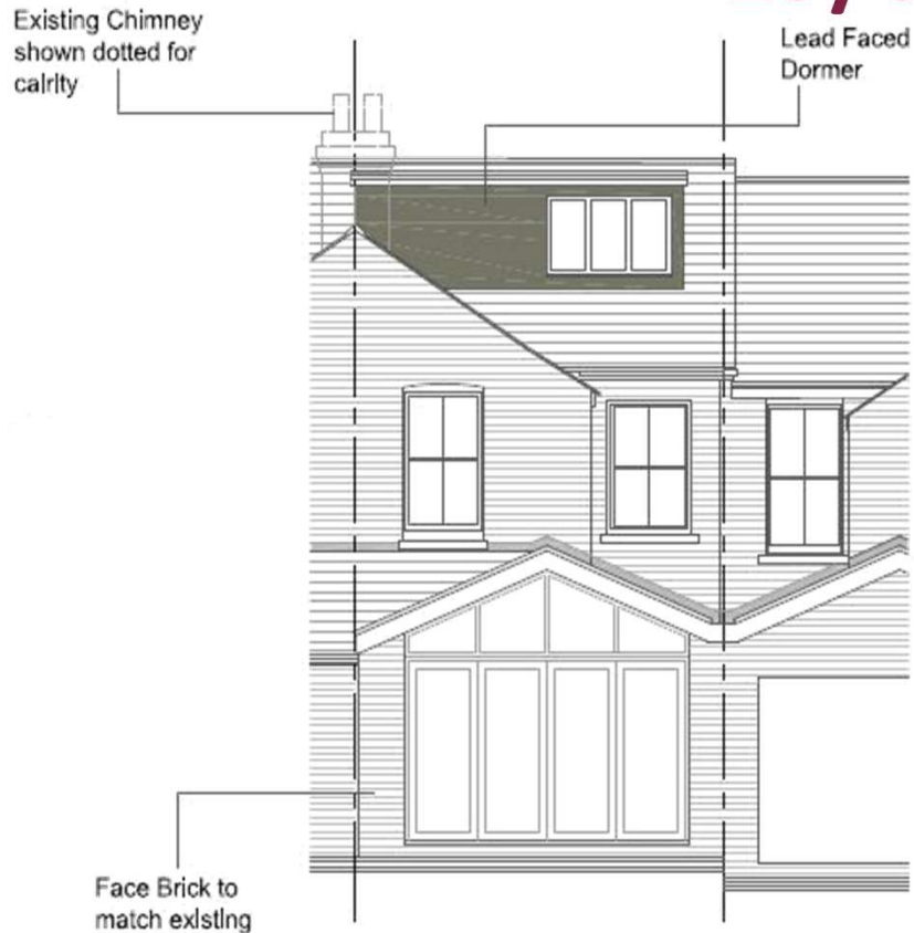
WEST ELEVATION (REAR)
